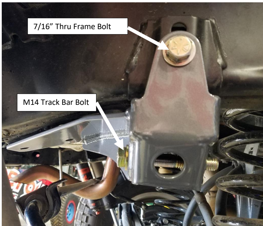
Figure 3. Synergy Rear Track Bar Frame Brace Bolt Locations
