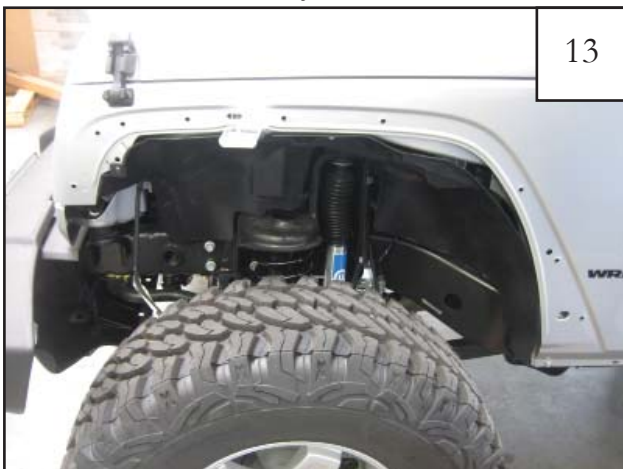
Hold splash shield up to inner wheel well to ensure that the edge is flush with the sheet metal. Remove from wheel well and trim or sand if splash shield extends beyond the sheet metal.
